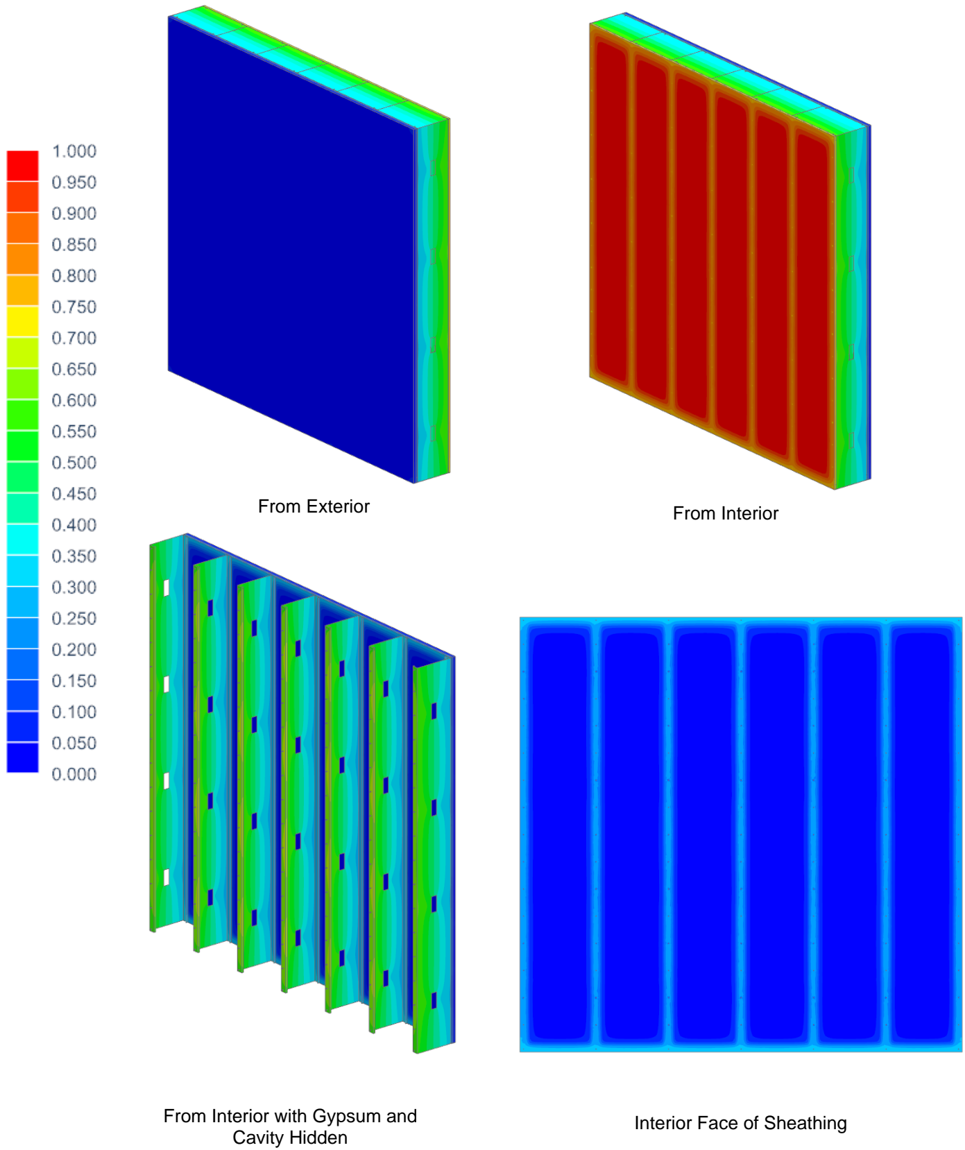
Figure C-3: Temperature Profiles for Interior Insulation Only Assembly #16, Fastener #1
