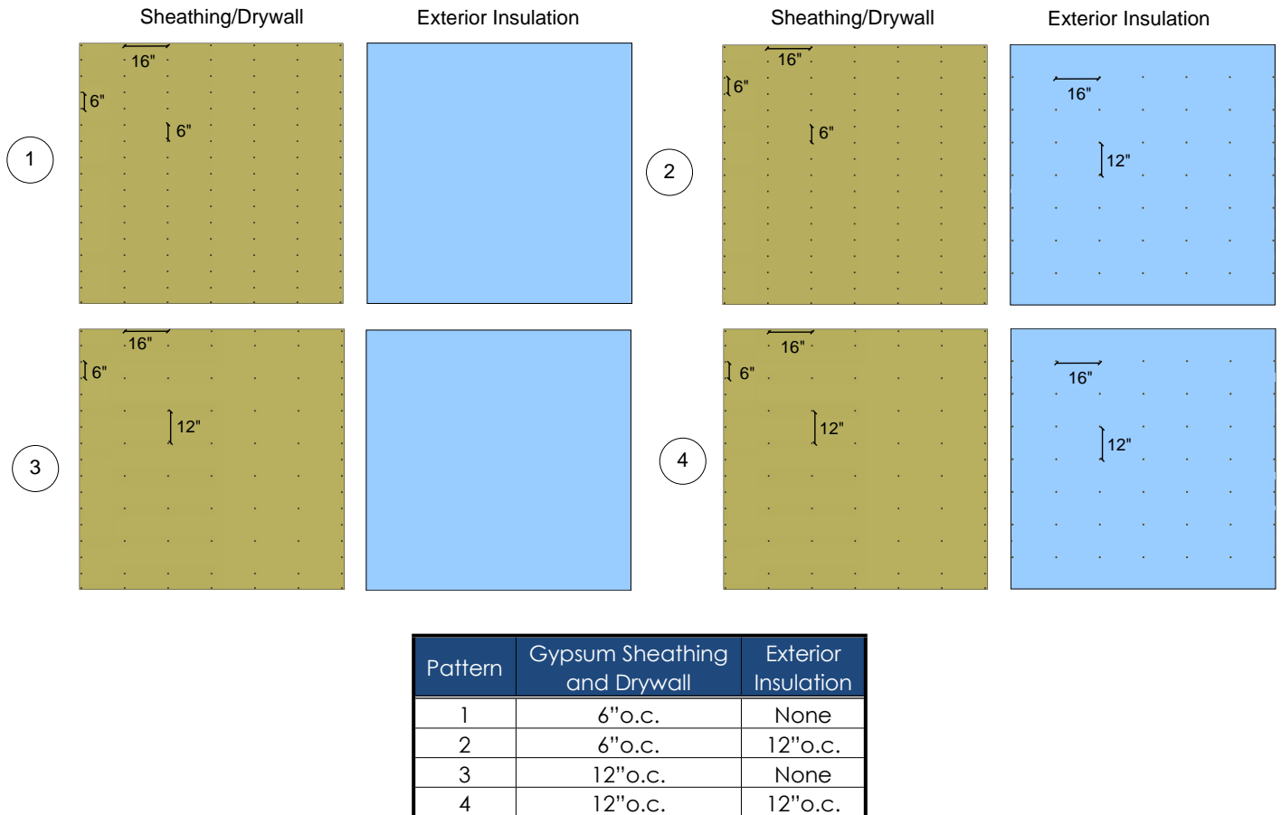
Figure 5-3: Fastener Patterns Analyzed for the Project Assemblies
