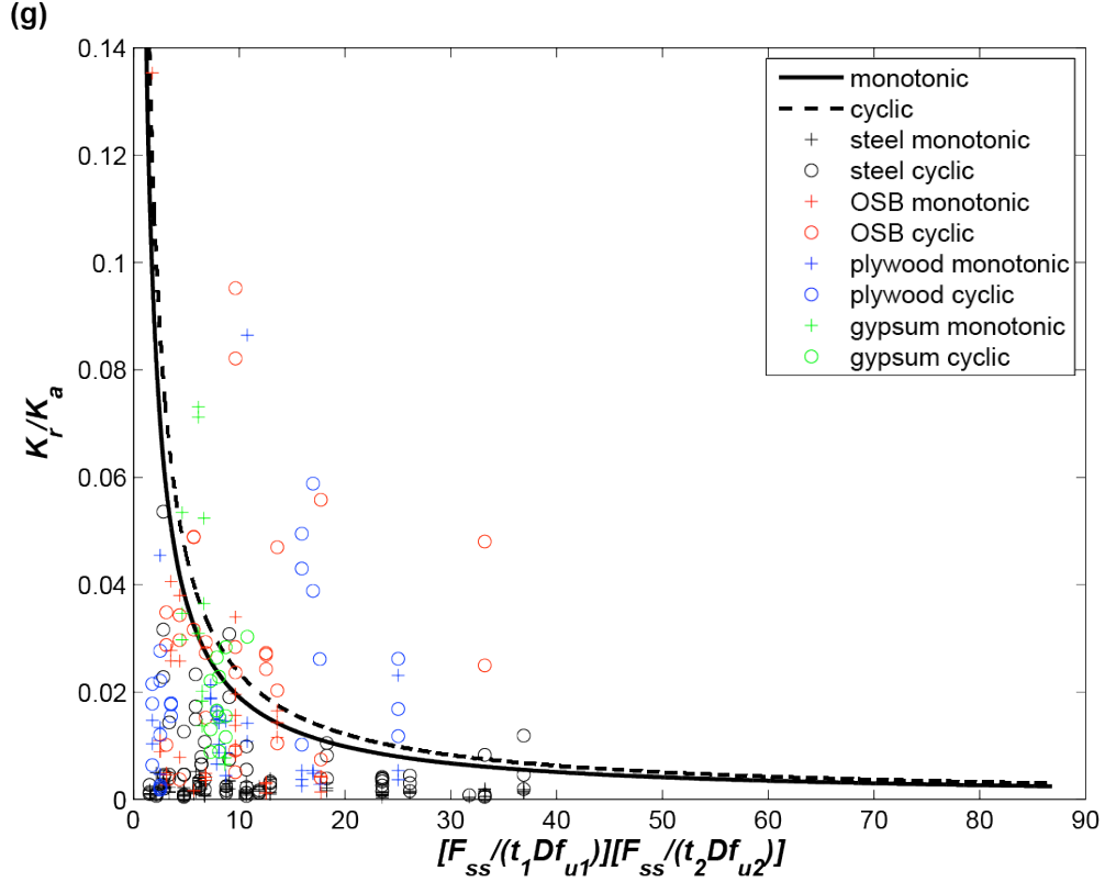
Figure 13: Steel and sheathing fastener backbone models: (a) F_y , (b) F_c , (c) F_r , (d) K_e , (e) K_s , (f) K_c , and (g) K_r
