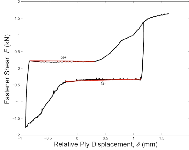
Figure 20: G+ and G- for cycle 5 of fastener configuration 1854-12-2
