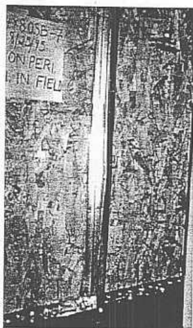
Interior stud buckling in OSB wall (cyclic tests)
