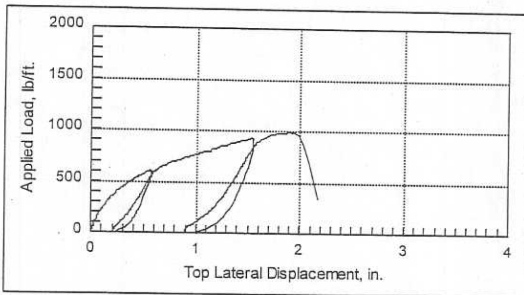
Fig. 6 Load vs. top of wall lateral displacement for specimen OSB-1A6
