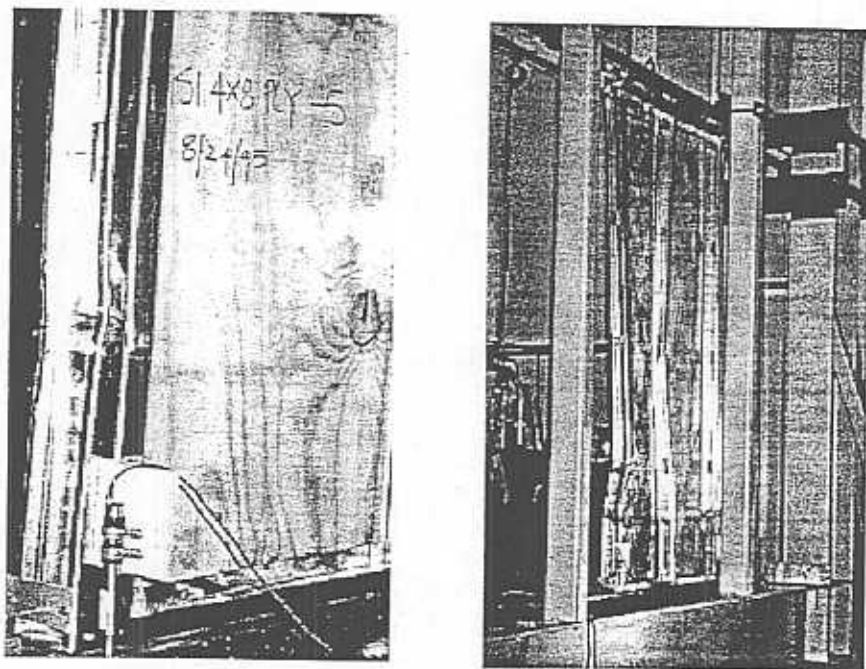
Chord stud failure in plywood walls (cyclic tests)
