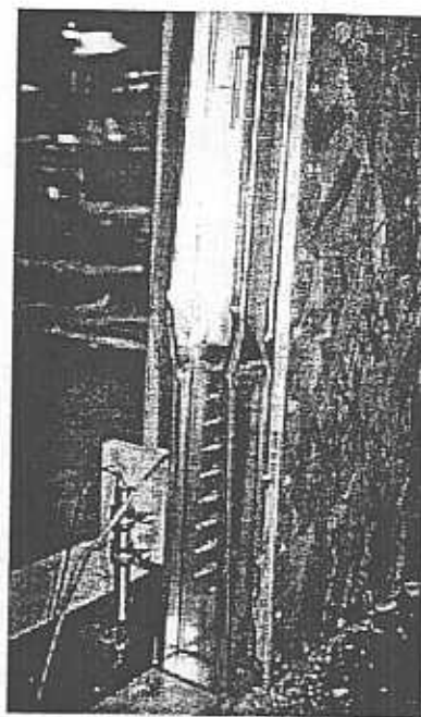
Chord stud failure in OSB walls (cyclic tests)
