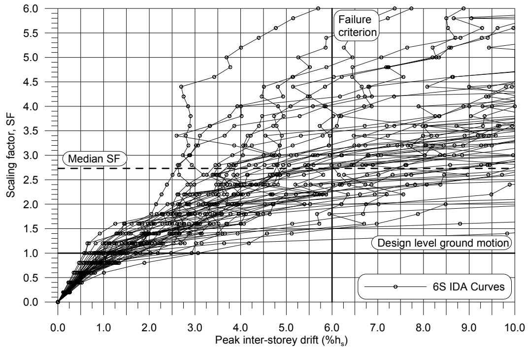
Figure I.9: IDA analysis for model 6S R_dR_0.2.6 -minbrace
