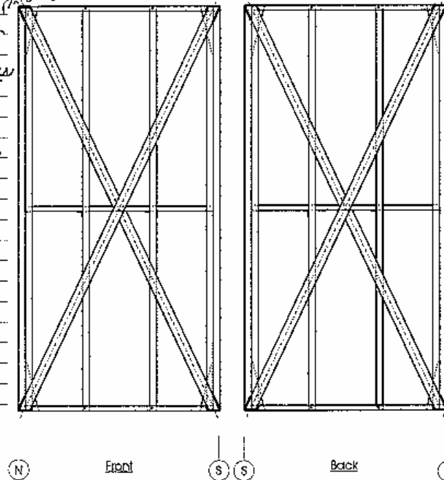
Figure E.6: Observations for test 15B-M
