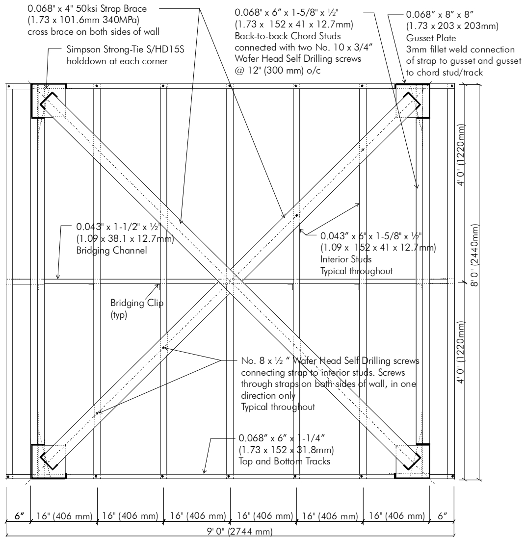
Figure B.37: Nominal dimensions and specifications for walls 21A-M and 22A-C
