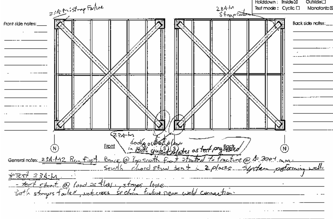
Figure E.18: Observations for test 23A-M
