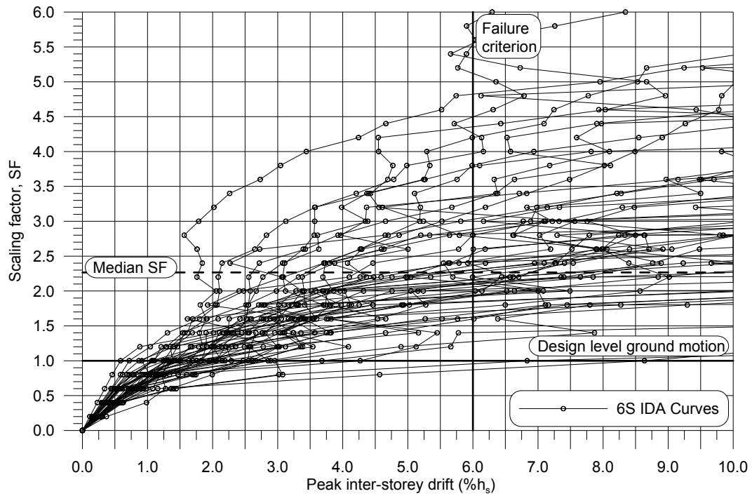
Figure I.13: IDA analysis for model 6S R_dR_o4 -minbrace
