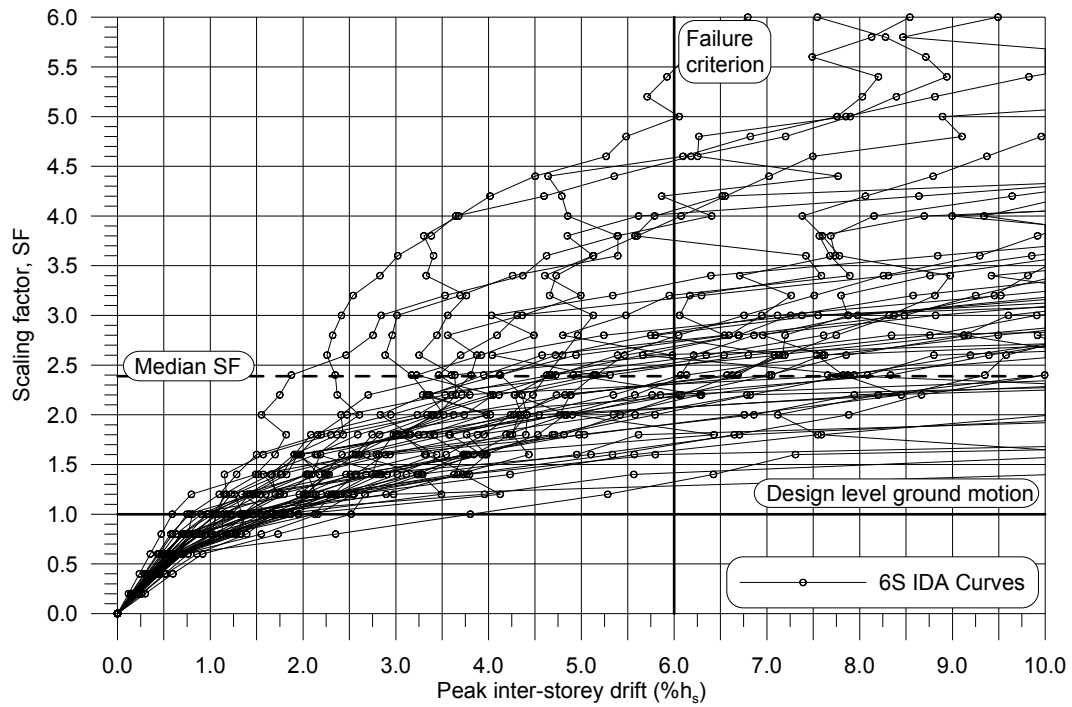
Figure I.11: IDA analysis for model 6S R d R 0.2.6 -2brace
