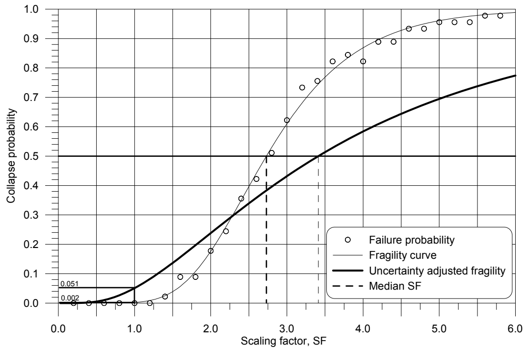
Figure I.10: Fragility curve for model 6S R_dR_0.2.6 -minbrace
