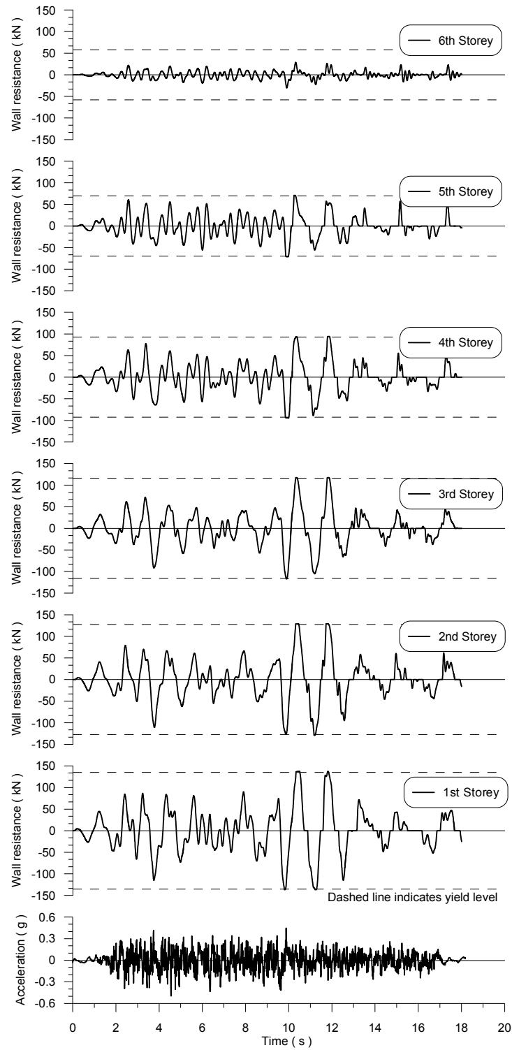
Figure H.6: Time history showing resistance vs. time for each storey, CM earthquake record, model 6S R_d R_o 2.6-minbrace
