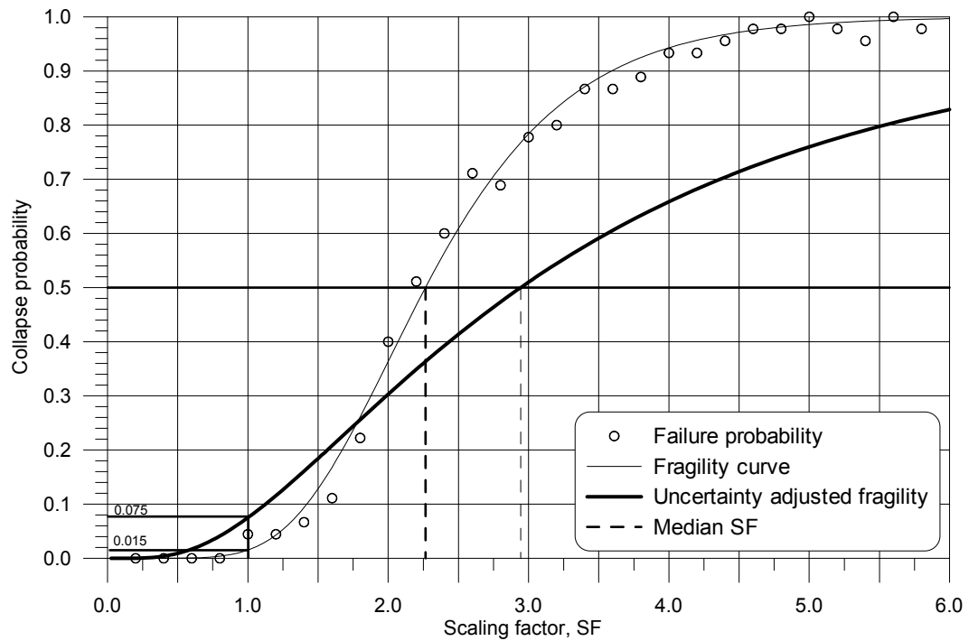
Figure I.14: Fragility curve for model 6S R_dR_o4 -minbrace
