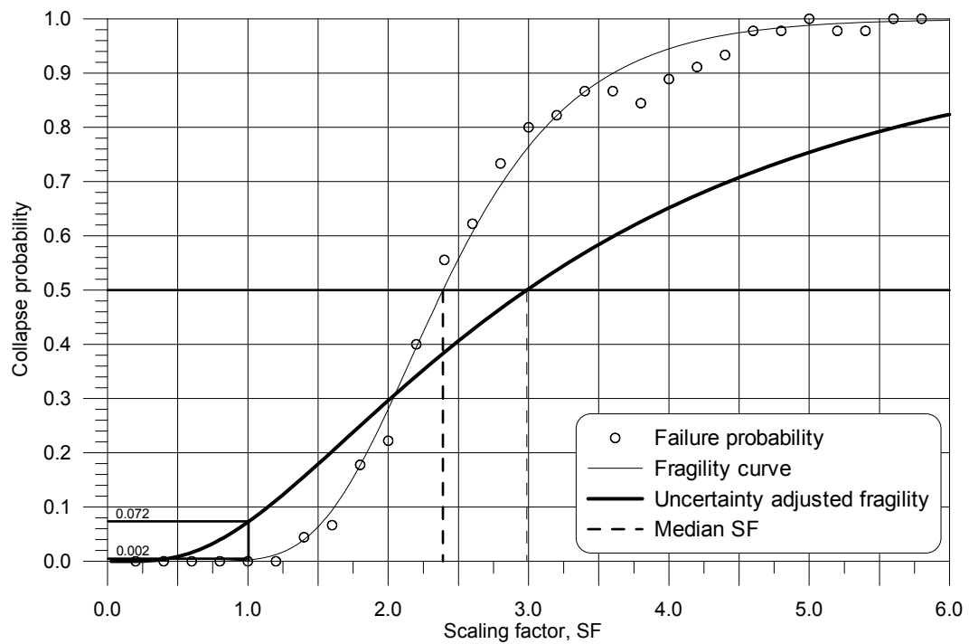
Figure I.12: Fragility curve for model 6S R d R 0.2.6 -2brace
