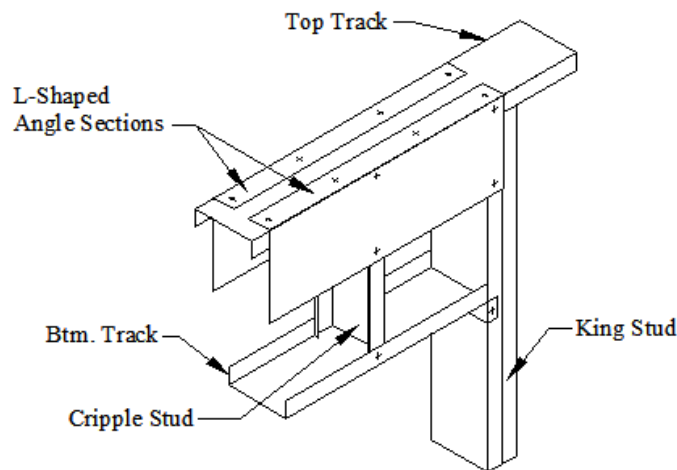
Figure 1.1 Double L-Header
