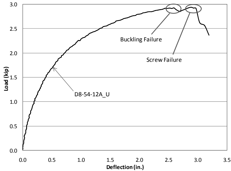
Figure 3.6 Uplift Load Case - Load-Deflection Curve Failure
