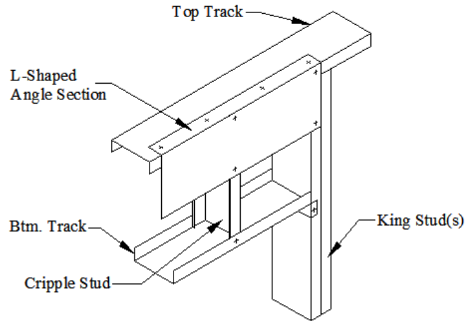
Figure 1.2 Single L-Header
