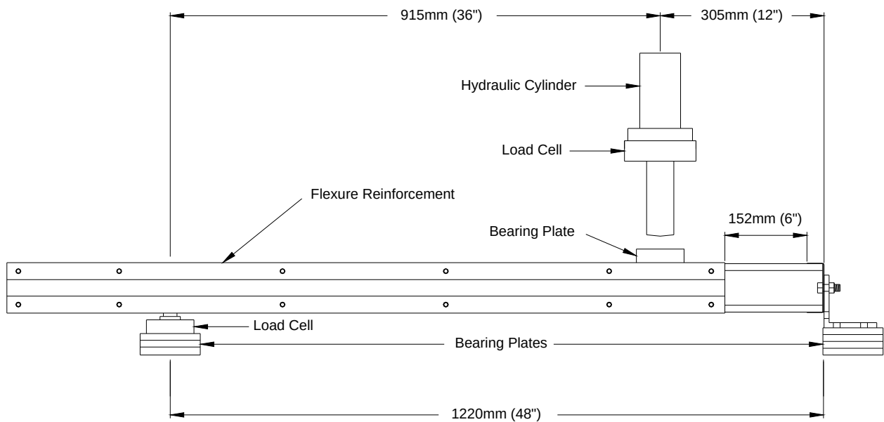
Figure 3-6: Schematic of a Typical Test Setup
