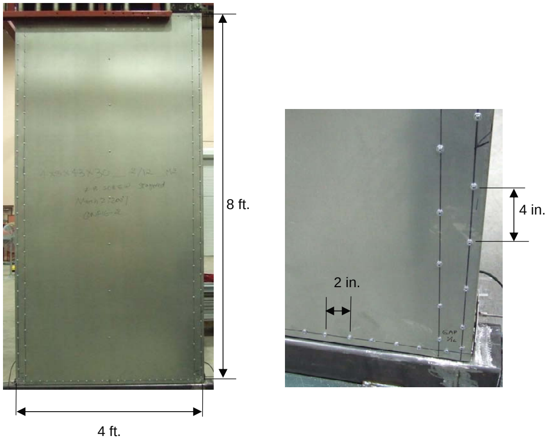
Figure 13 Staggered screw pattern (2"/12")
