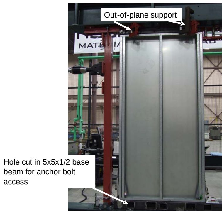
Figure 2 Back view of the test setup
