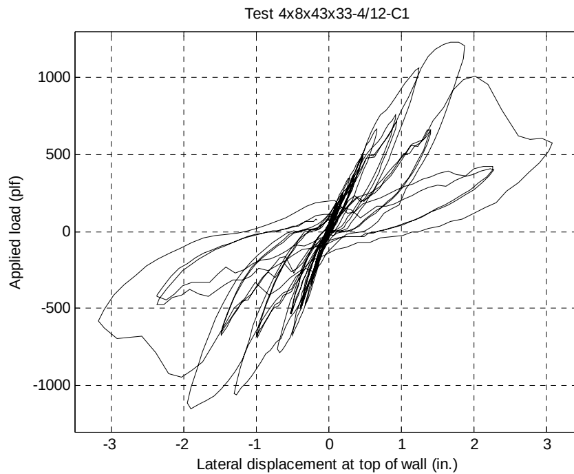
Figure 16 Observed hysteresis curve for test 4 \times 8 \times 43 \times 33-4/12-C1
