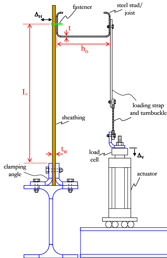
Figure 4 Basic test setup (line drawing)
