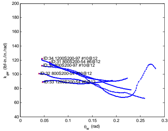
(a) OSB sheathing stiffness, tangent k_{\phi_w}
