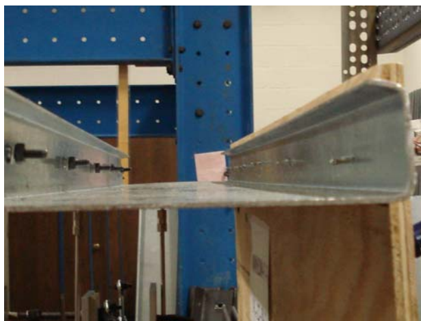
typical sheathing-joist fastener alignment, 2 out of 5 noted as mis-aligned for this specimen
