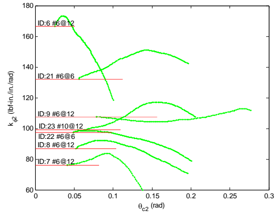
(b) connector stiffness, tangent k_{\phi_{c2}}
