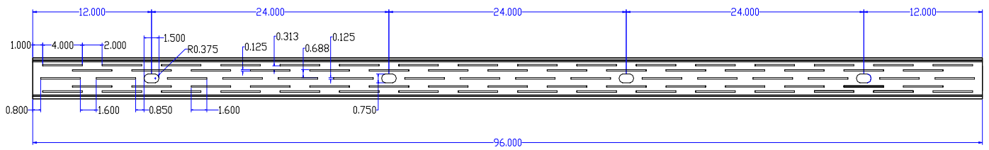
Figure 16 – Slit-Web Stud Configuration and Dimensions
