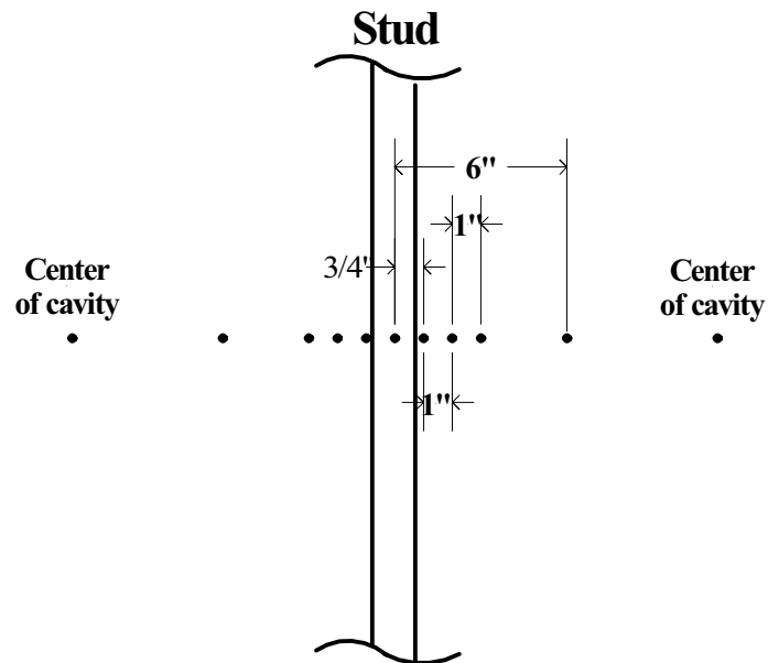
Figure 12 - Stud Array TC Layout
