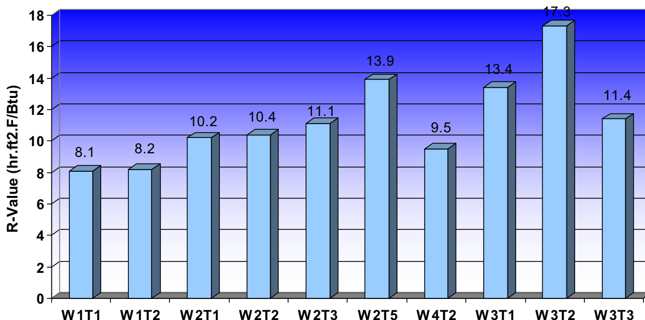
Figure 19 - Surface-to-Surface R-Values (Phase I)
