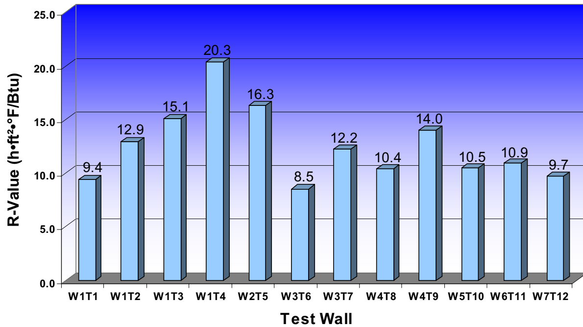
Figure 21 - Surface-to-Surface R-Values (Phase II)
