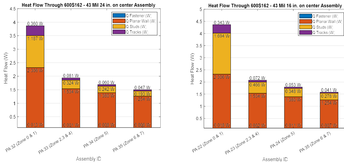
Figure 19: Comparison of Heat Flow through 600S162 - 43 Mil 24 in. on center and 600S162 - 43 Mil 16 in. on center Assemblies
