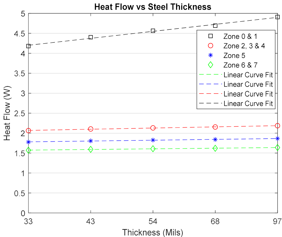
Figure 13: Heat Flow vs Steel Thickness for Different Climate Zones
