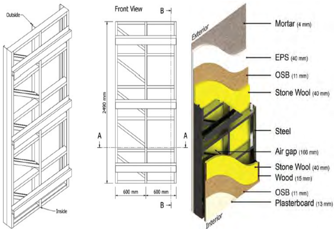
Figure 2: Description of CFS Wall Assembly and Components used by Santos et al
