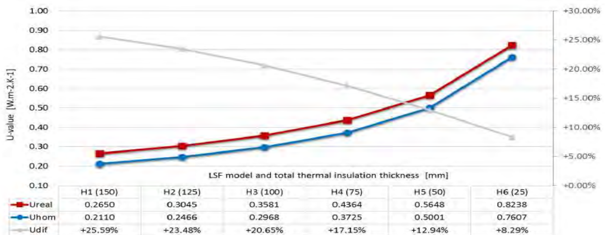
Figure 5: Results of the Hybrid Frame Construction Parametric Study (Roque and Santos)
