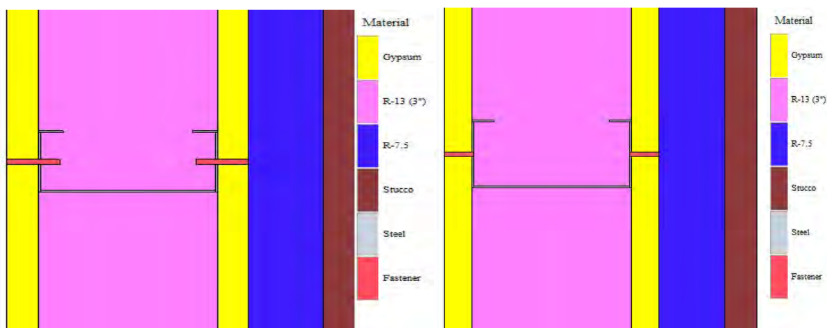
Figure 11: 2-D Section Cut through Wall Assembly at Fastener Locations (Left – Fastener length modelled and Right – Fastener modelled from start of sheathing to interior of Flange)
