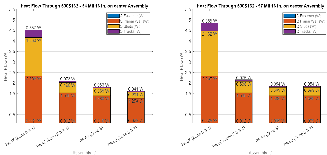
Figure 22: Heat Flow through 600S162 - 54 Mil 16 in. on center and 600S162 - 97 mil 16 in. on center Assemblies
