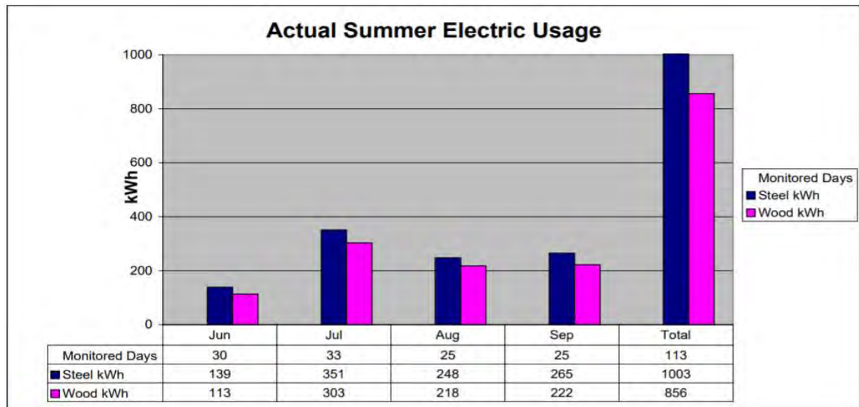
Figure 8: Comparison of Summer Electric Usage (NAHB Report)
