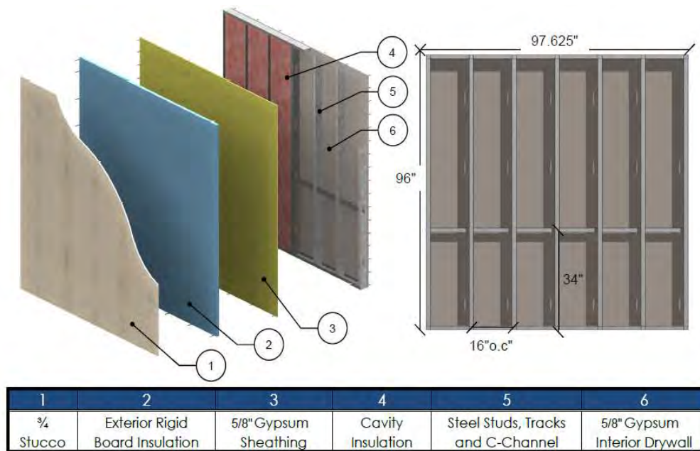
Figure 1: Basic configuration of the project assemblies (RP18-1)
