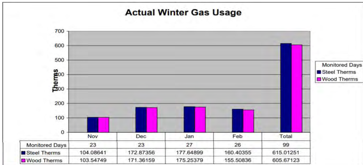
Figure 9: Comparison of Winter Gas Usage (NAHB) Report
