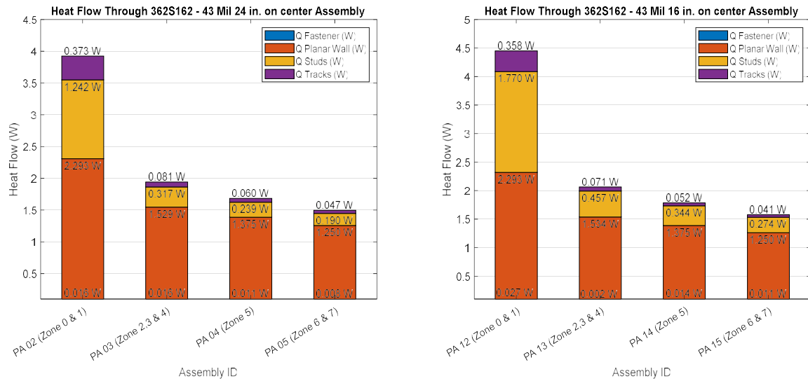
Figure 18: Comparison of Heat Flow through 362S162 - 43 Mil 24 in. on center and 362S162 - 43 Mil 16 in. on center Assemblies
