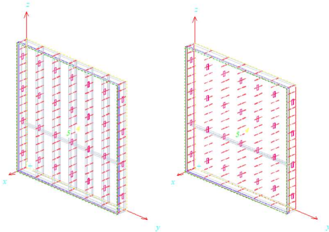
Figure 12: Left to Right, Heat3 Model of Wall Assembly with CFS Studs & Heat3 Model of Wall Assembly without CFS Studs
