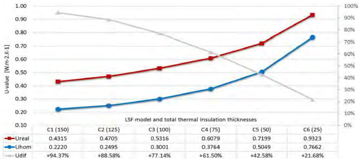
Figure 4: Results of the Cold Frame Construction Parametric Study (Roque and Santos)
