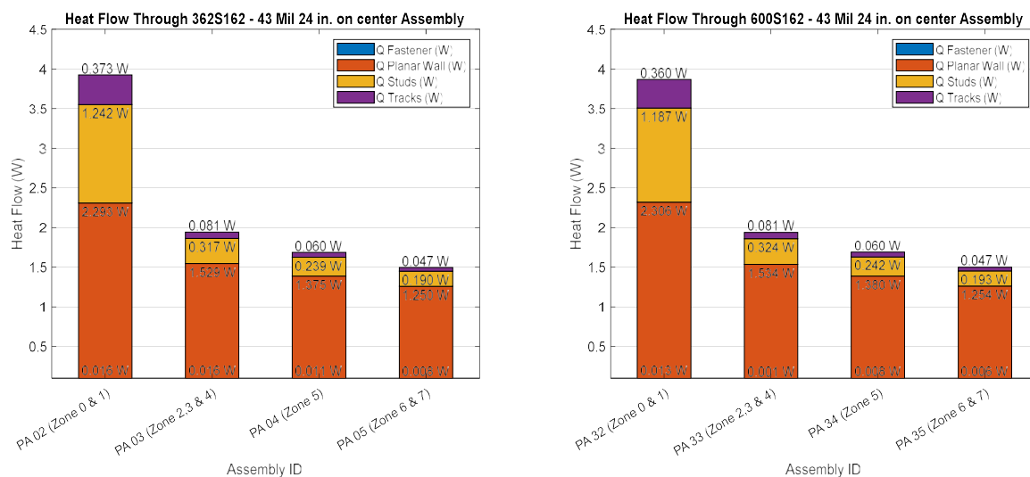
Figure 14: Comparison of Heat Flow through 362S162 - 43 Mil 24 in. on center and 600S162 - 43 mil 24 in. on center Assemblies
