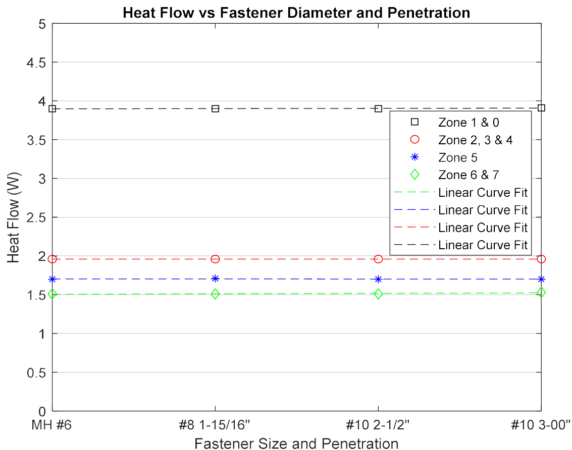
Figure 23: Heat Flow vs Fastener Diameter and Penetration for Different Climate Zones
