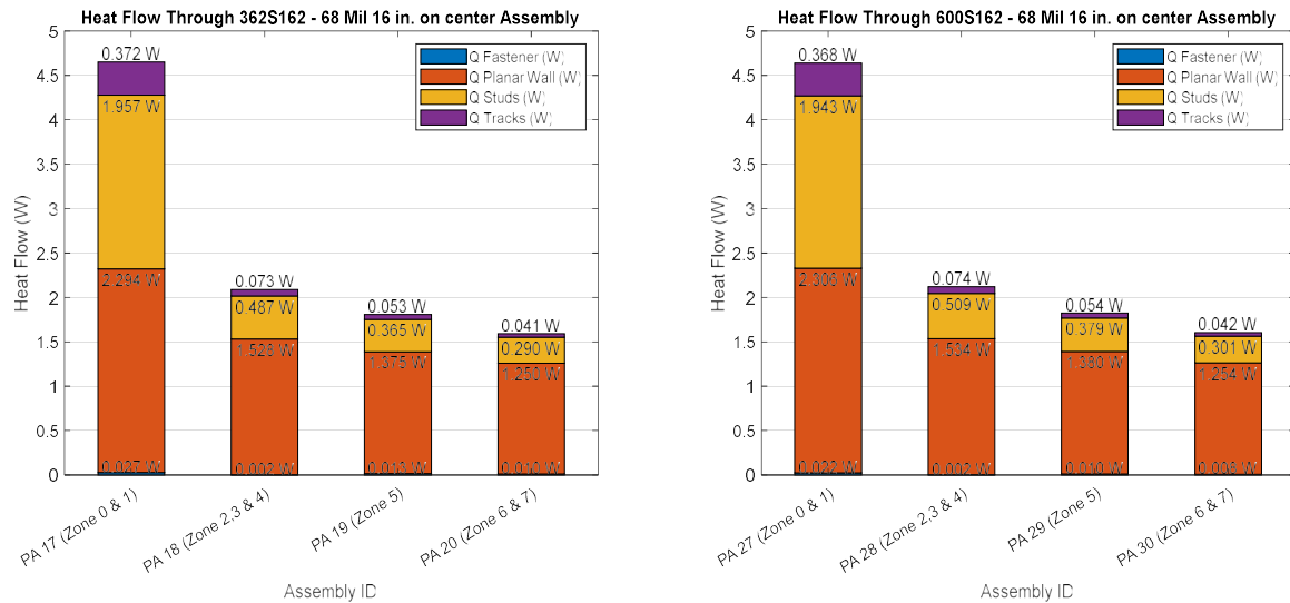
Figure 17: Comparison of Heat Flow through 362S162 - 68 Mil 16 in. on center and 600S162 - 68 mil 16 in. on center Assemblies
